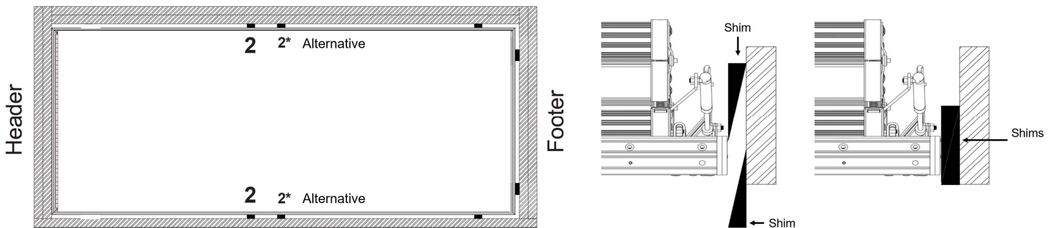
FIGURE 25 : SHIMMING SIDE FRAME
