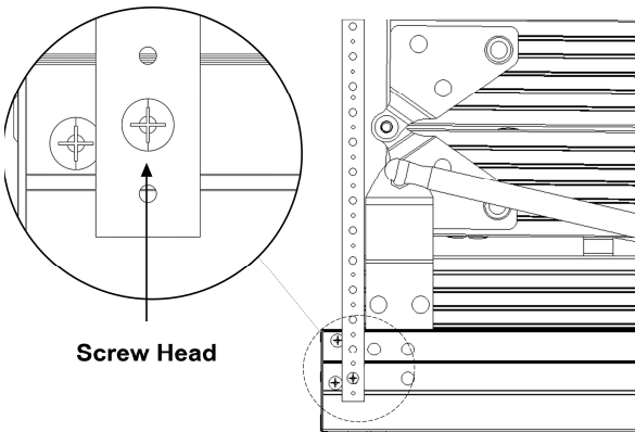
FIGURE 6: STRAP POSITION
