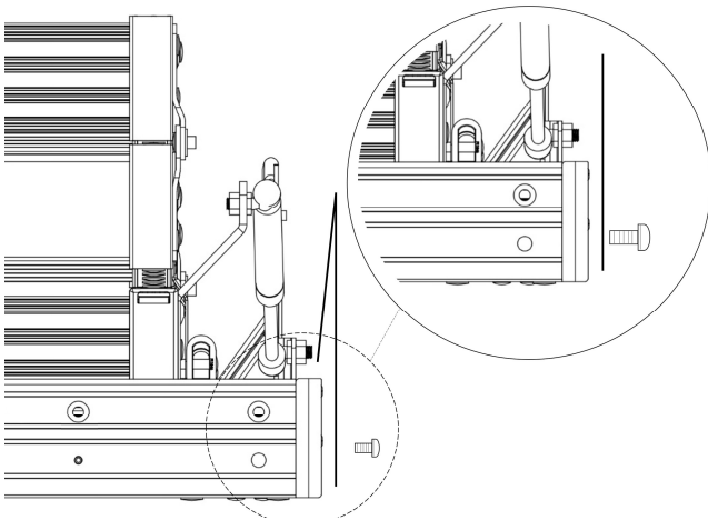
FIGURE 5 : STRAP INSTALLATION
