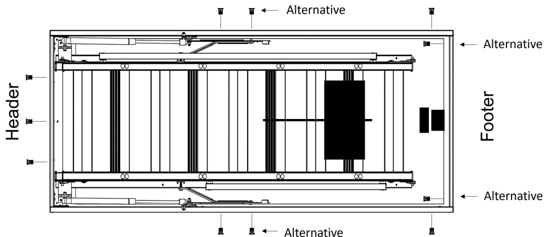
FIGURE 4: BUSHING LOCATIONS
