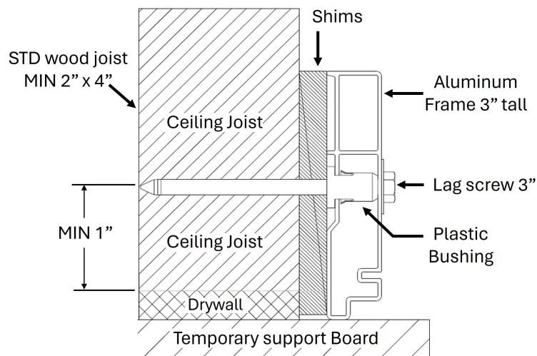
FIGURE 2 CEILING JOIST REQUIREMENTS
