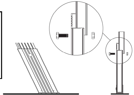
FIGURE 29 ALUMINUM FOOT INSTALLATION
