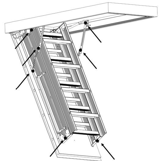
FIGURE 34 : LUBRICATION POINTS
