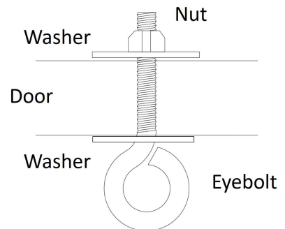
FIGURE 21 : ATTACHING EYEBOLT
